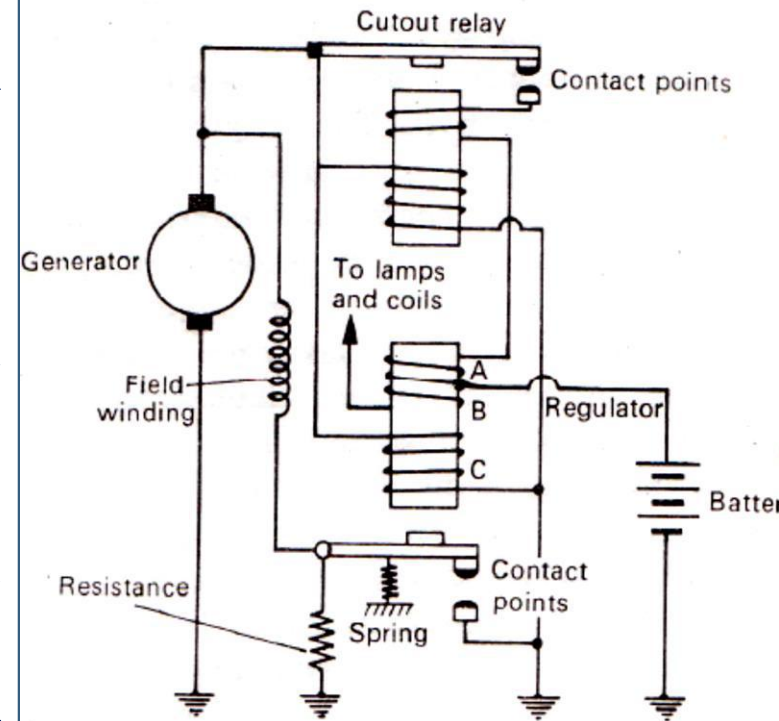
Fig. 5.10 Circuit diagram of a typical compensated voltage regulator with cutout relay.
