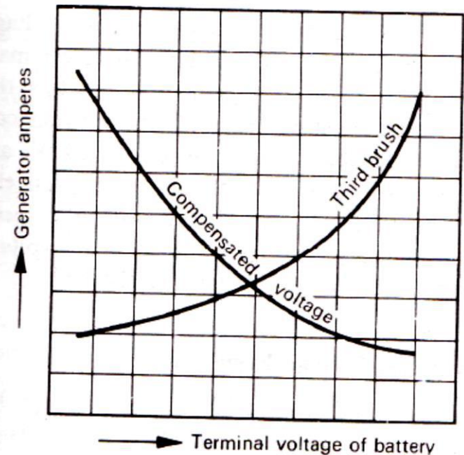
Fig. 5.12 Comparison of third-brush and compensated voltage system.
