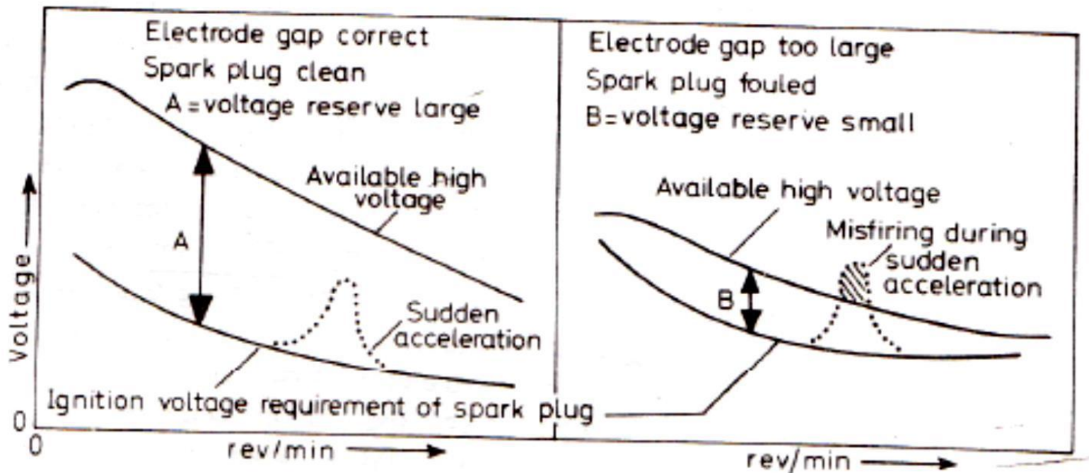
Fig. 8.6 Curves of ignition voltage requirements of spark plug (courtesy: MICO).
