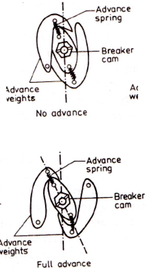
Fig. 7.18 Centrifugal advance mechanism in full and advance positions.
