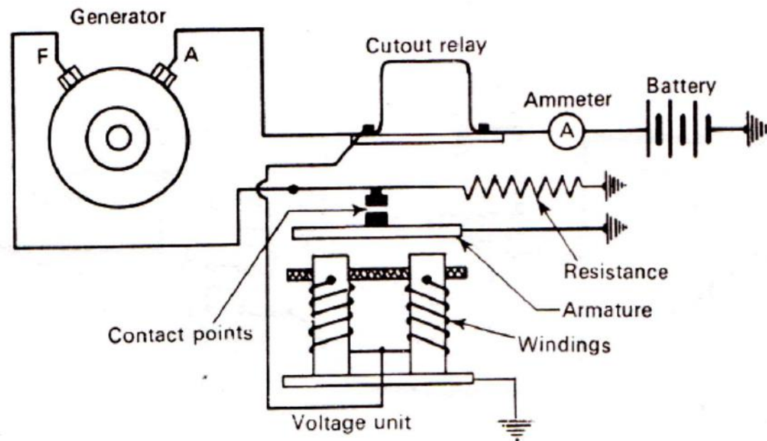
Fig. 5.6 Wiring diagram of the step voltage control unit and cutout relay.
